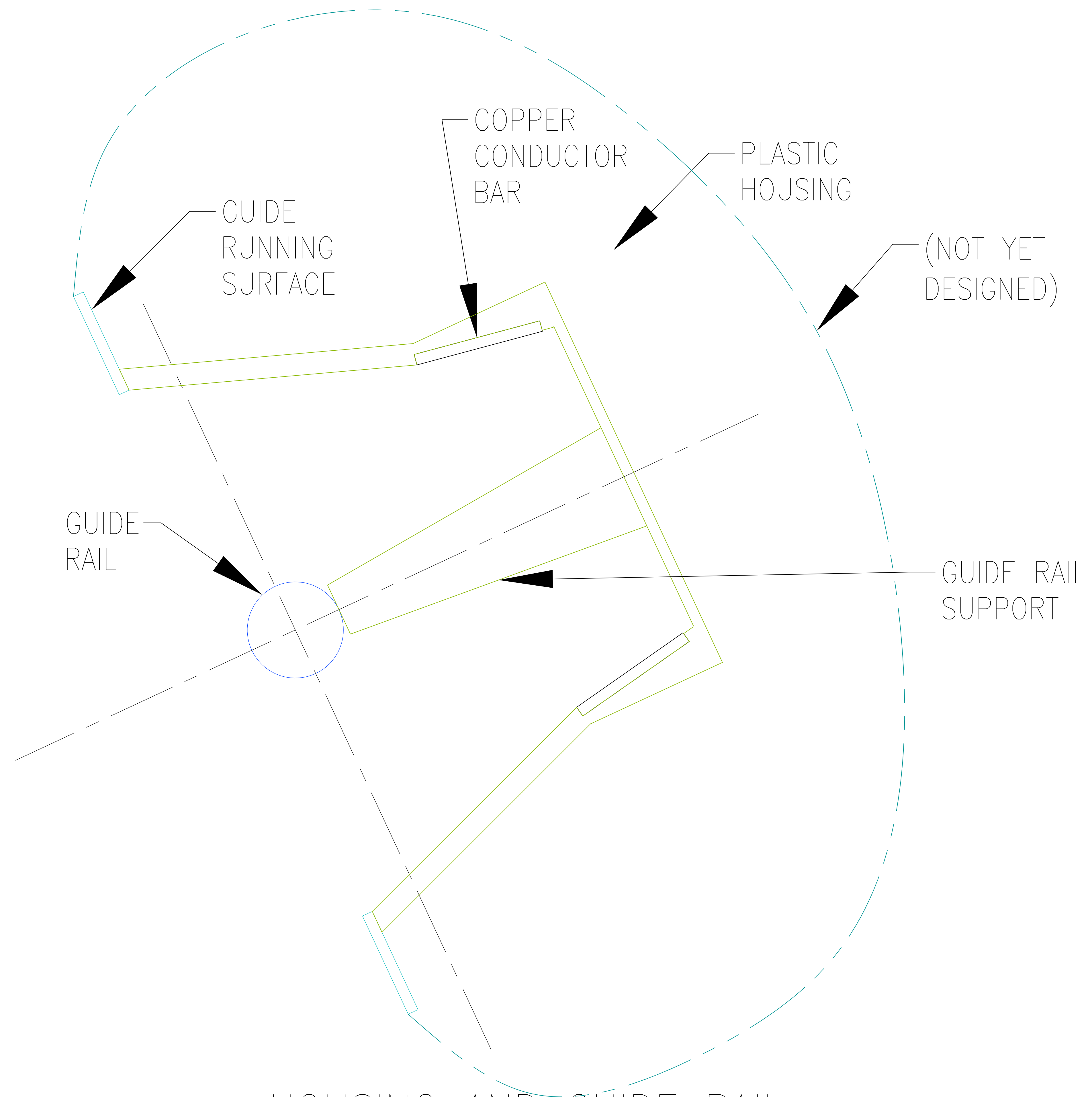
HOUSING AND GUIDE RAIL - FULL LENGTH OF TRACK
