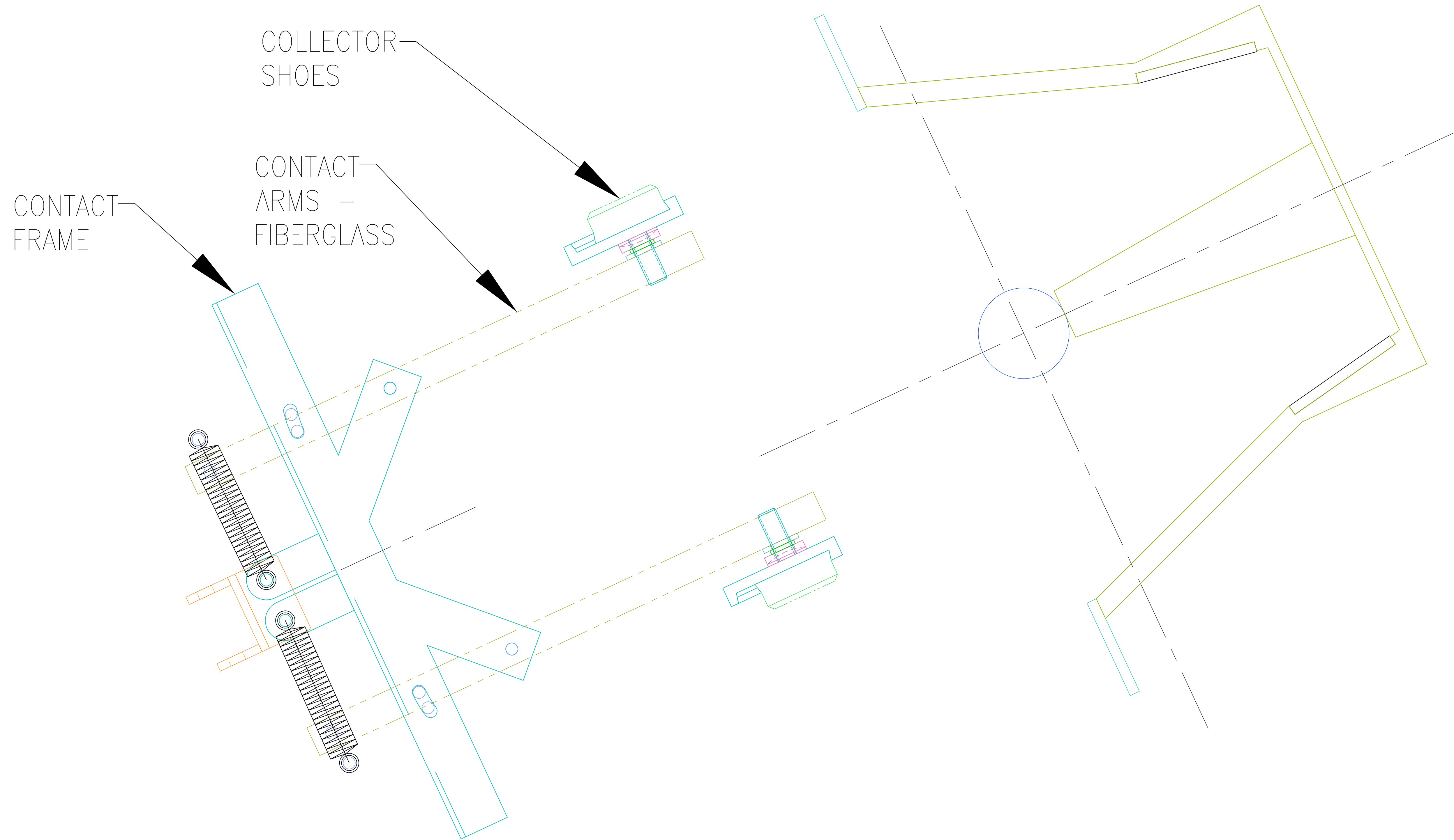
TRACK AND CONTACT ASSEMBLIES - DISENGAGED
